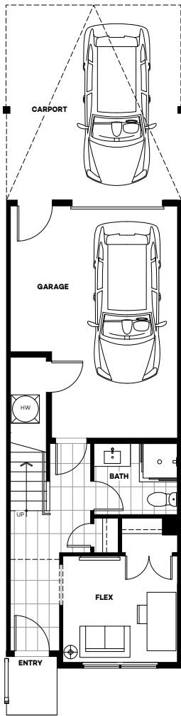
LOWER FLOOR
